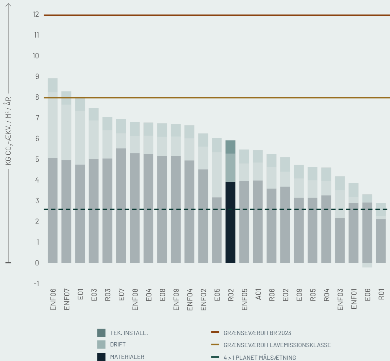
Figur R02.5: Boligcases
