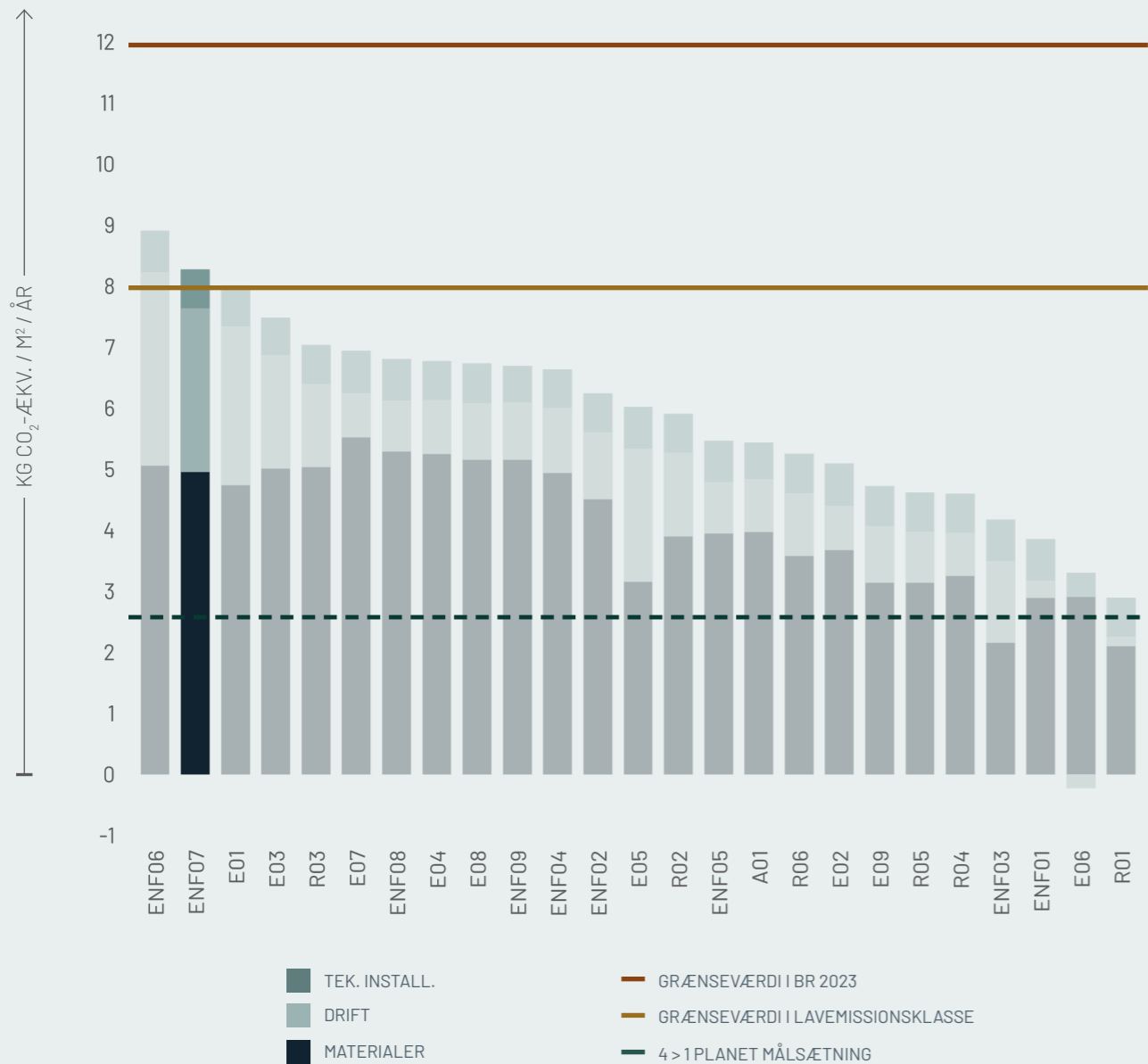
Figur ENF07.5: Boligcases
