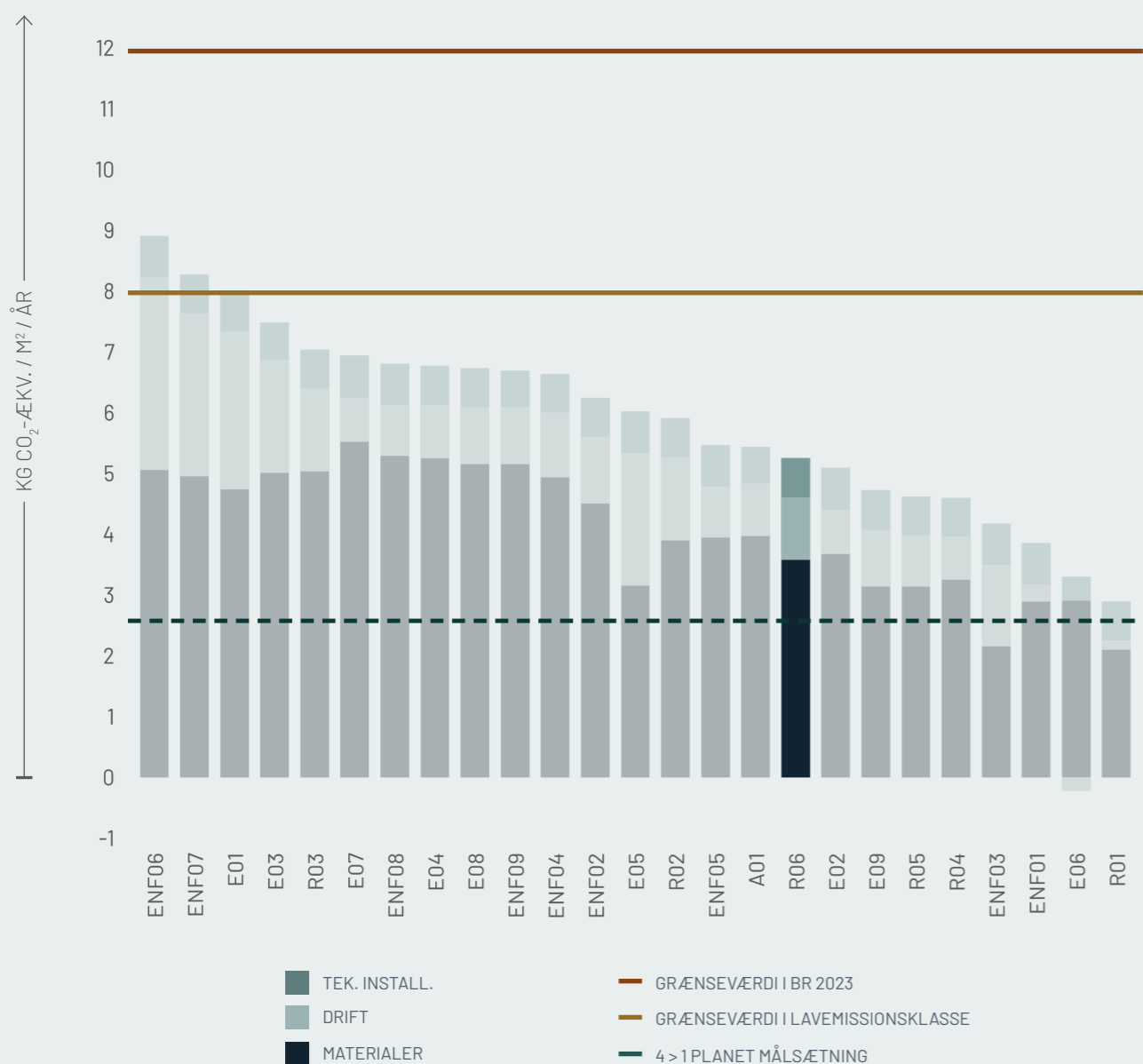
Figur R06.5: Boligcases
