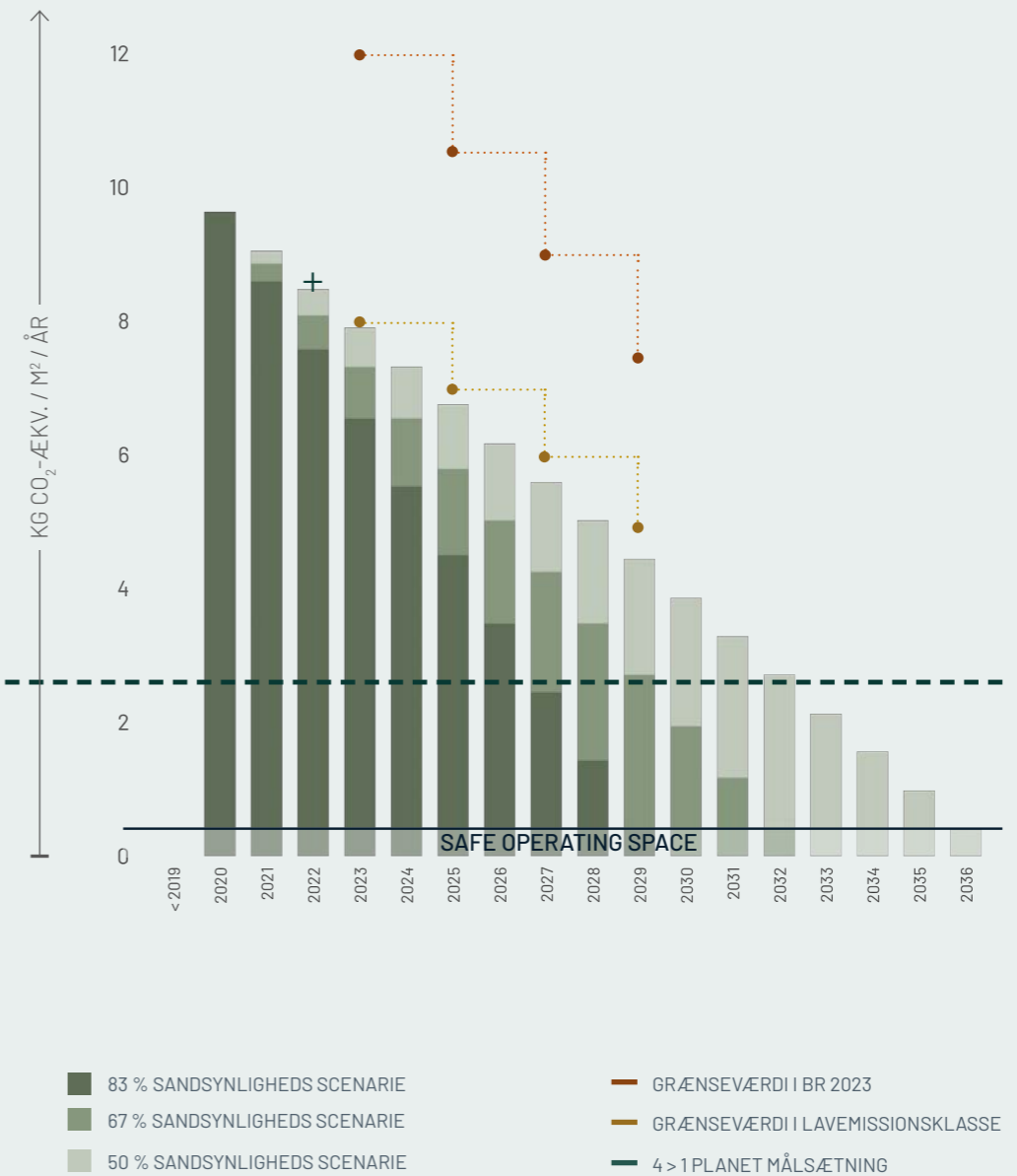
Figur ENF06.6: Reduction Roadmap
