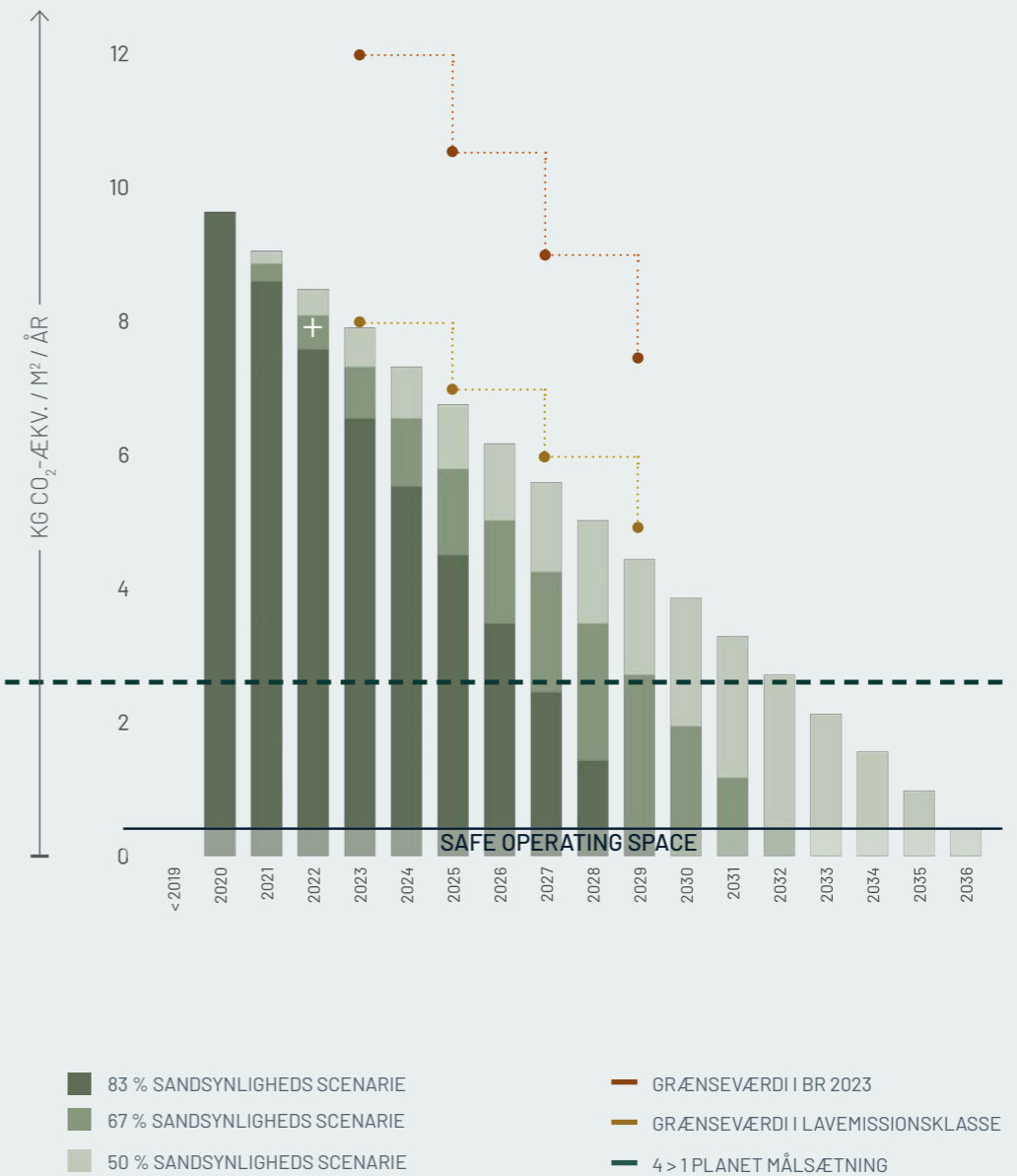
Figur E01.6: Reduction Roadmap
