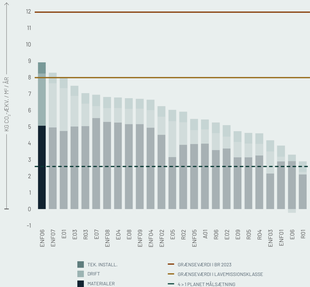
Figur ENF06.5: Boligcases
